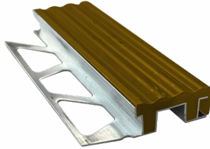
Basamak Profili - Esnek PVC Bantlı Stair Edge Trim - Pvc Strip (Flexible) Insert 11 mm
